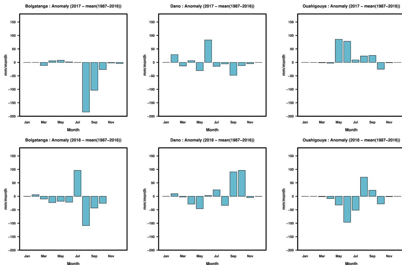
Fig. 2. Monthly anomaly (2017/2018 – mean (1987–2016)) of total rainfall amount for Bolgatanga, Dano and Ouahigouya.
