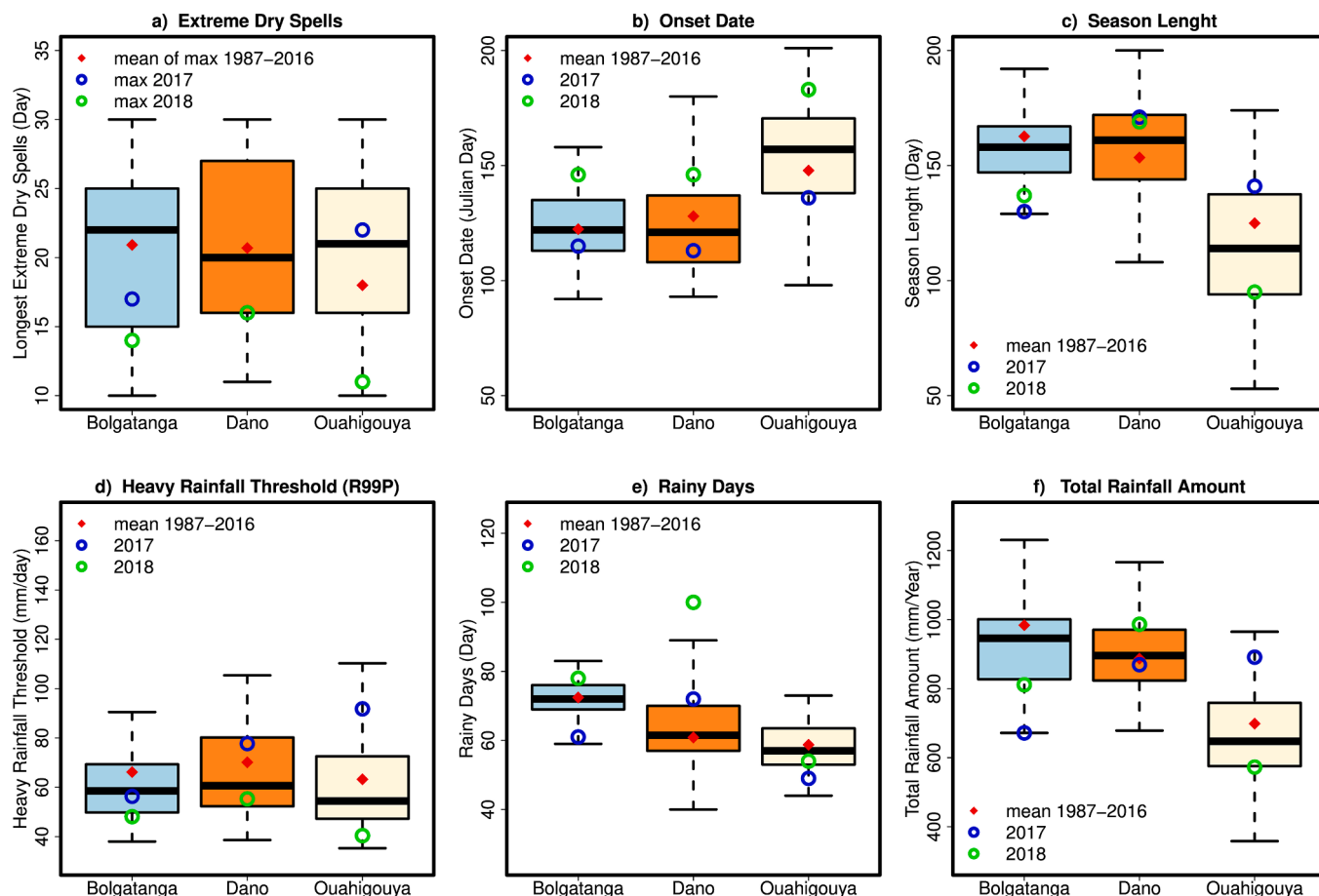
Fig. 5. Historical distribution of some pluviometric extreme events in Bolgatanga (light blue), Dano (chocolate), and Ouahigouya (cornsilk). a) Longest intra-seasonal extreme dry spells (day); b) Onset date (Julian day); c) Season length (day); d) Heavy rainfall threshold (mm/day); e) rainy days (day) and f) total rainfall amount (mm/year). The red-filled diamond represents the mean of the normal year (1987–2016); the circles 2017 (blue) and 2018 (green) represent observed values of each extreme. (For interpretation of the references to colour in this figure legend, the reader is referred to the web version of this article.)
