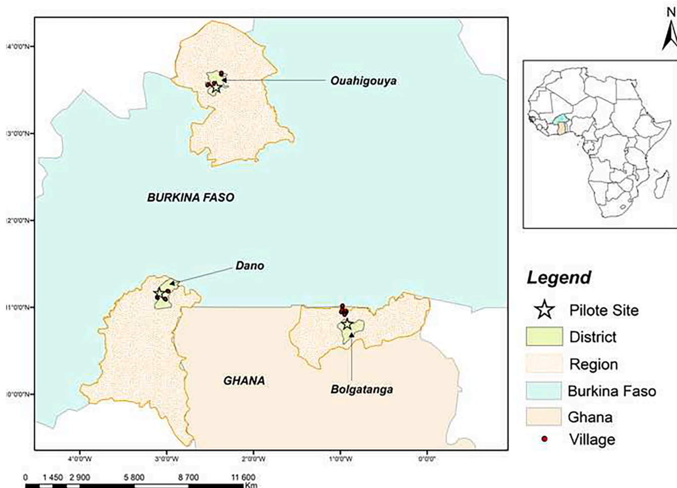
Fig. 1. Location Map of Bolgatanga, Dano and Ouahigouya.
