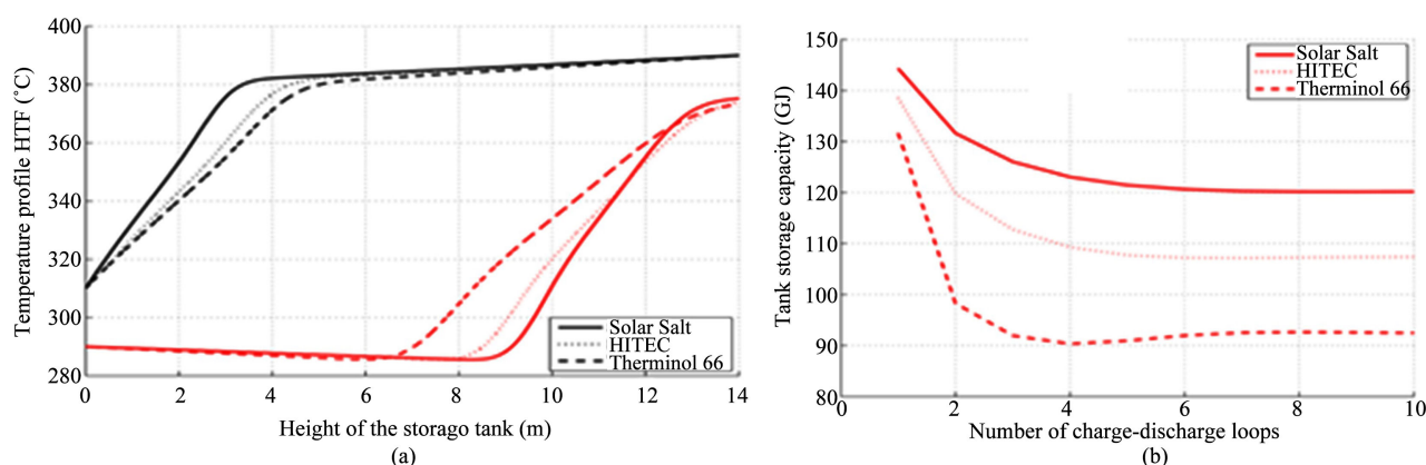
Figure 7. Temperature profile for different HTFs (a), tank storage capacity for different HTFs (b) [57].
