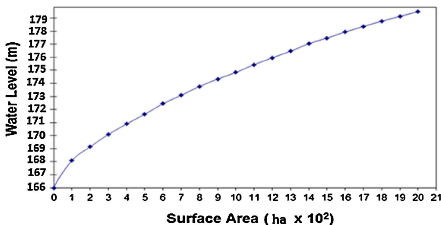
Fig. 3. Relationship between the Tono dam water levels (above mean sea level) and the Surface Area (provided by ICOUR).
