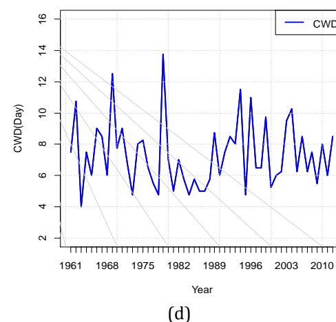
Figure 3: Inter-annual trends of the rainfall indices from 1961 to 2012: a) Total annual precipitation; b) Maximum 1 day precipitation; c) Consecutive Dry Days; d) Consecutives Wet Days
