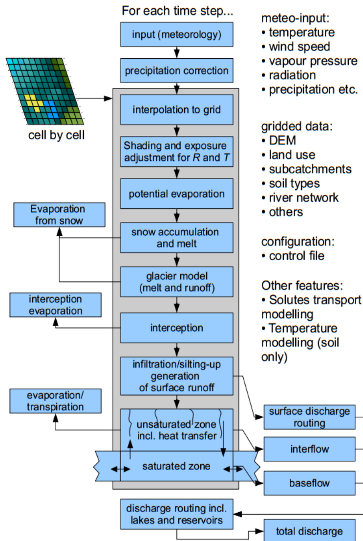
Figure 3-4: Flow chart of the WaSiM model. Blue boxes indicate the sub-models
