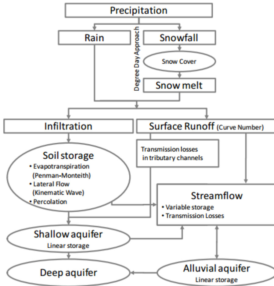
Figure 3-3: Flow chart of the SWAT model after Busche (2012)
