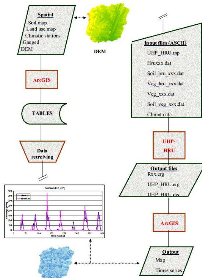
Figure 3-2: Flow chart of the UHP-HRU model
