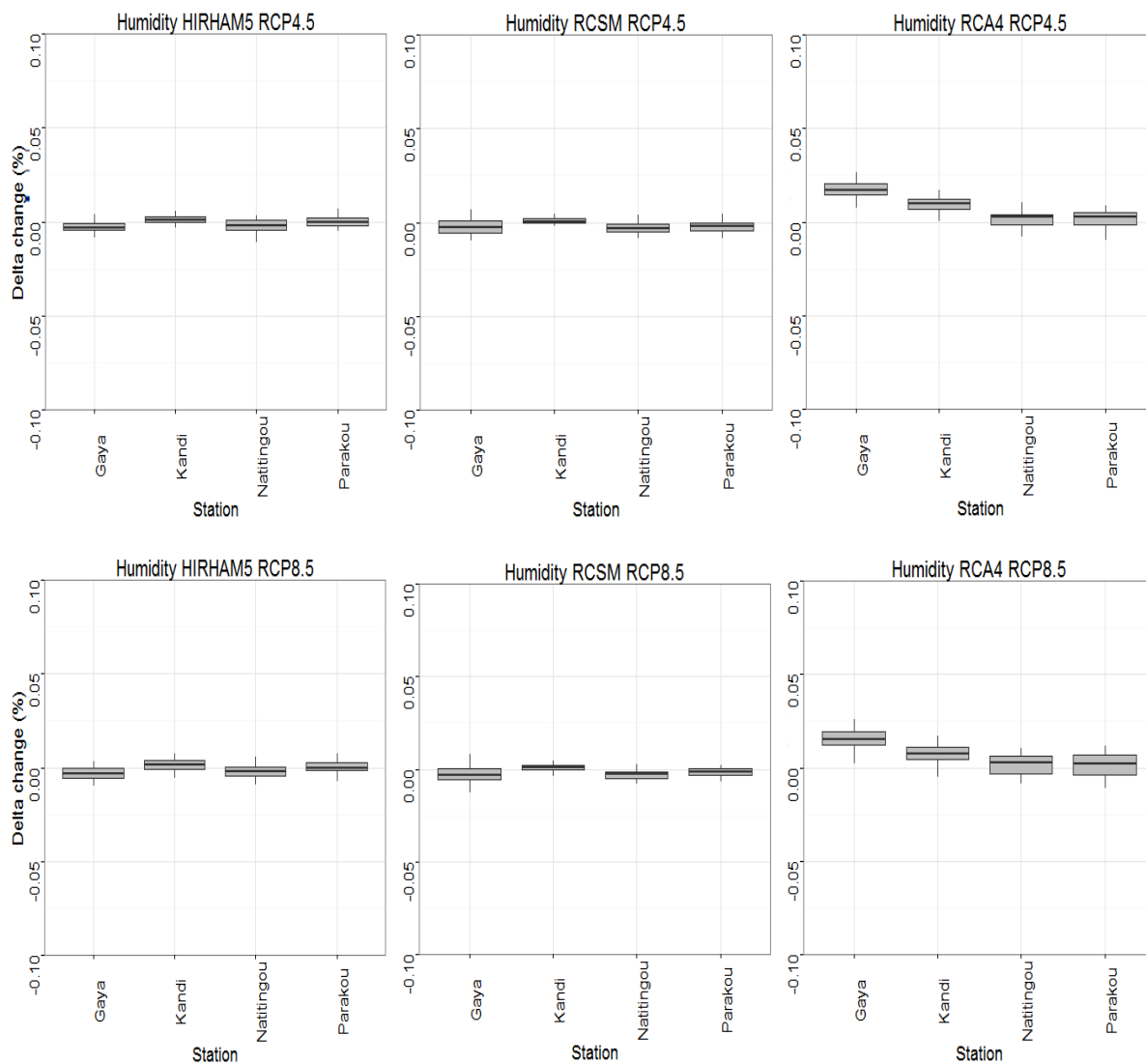
Figure C.2: Relative humidity
