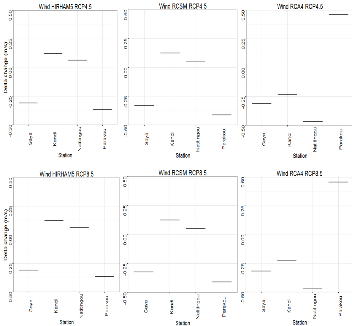
Figure C.3: Wind speed
