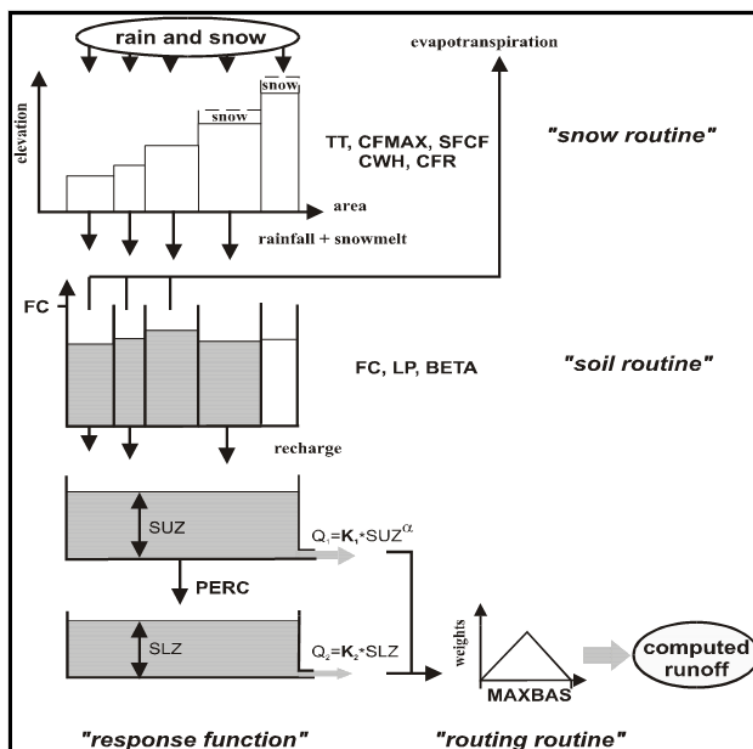
Figure 3-1: Structure of the standard version of the HBV-light model
