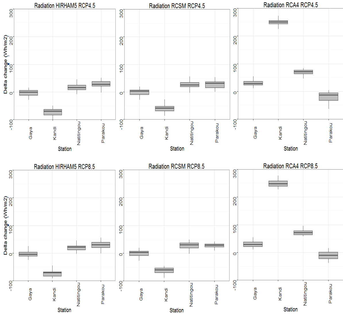
Figure C.1: Annual radiation
