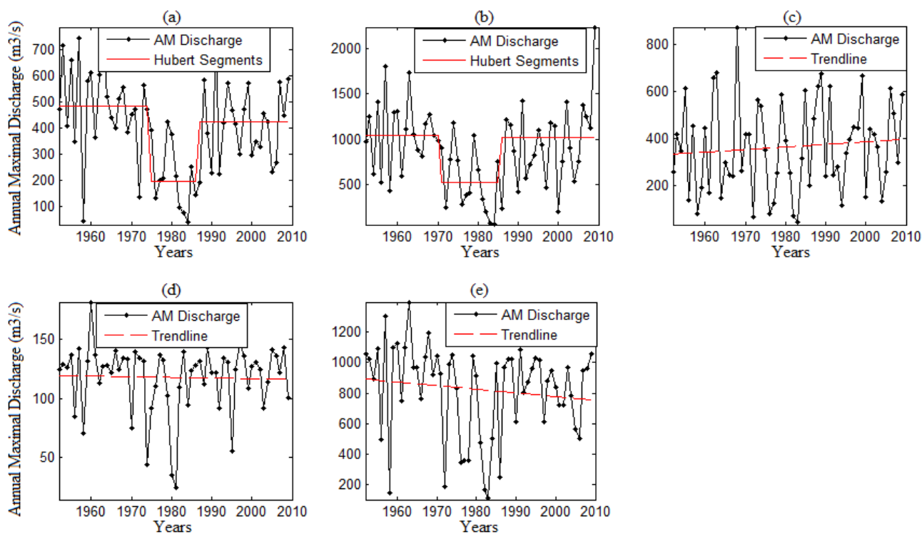
Figure 3-2: Plot of the annual maximal discharge and the corresponding linear trend line or Hubert segments at each station: (a) Bétérou, (b) Savè, (c) Atchérigbé, (d) Domè, and (e) Bonou.
