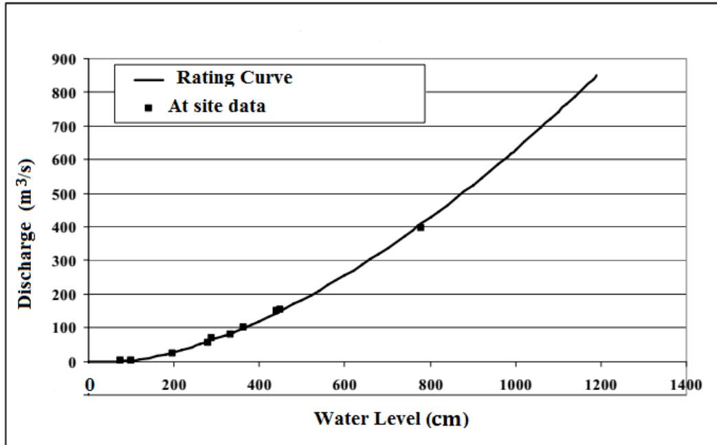
Figure 2-5: Water level discharge relationship for Zou catchment at Atchérigbé gauge (DGEau, 2008), valid from 1997 up to date.
