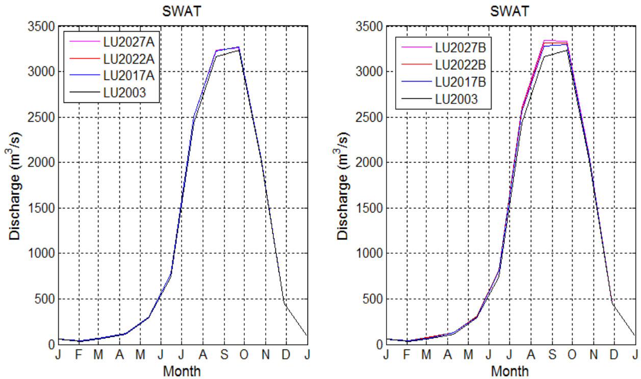
Figure 6-5: Mean monthly discharge simulated by SWAT for the different land use scenarios.
