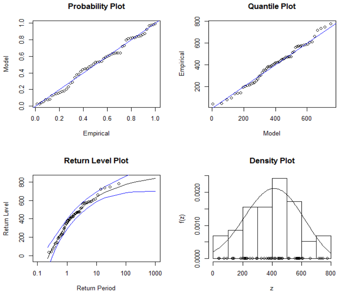
Figure 3-3: Diagnostic plots for the GEV-0 fit to the Bétérou station annual maximum discharge.
