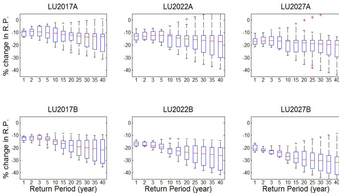
Figure 6-13: Percentage change in return period compared to the baseline as computed from WaSiM for the different scenarios and time windows
