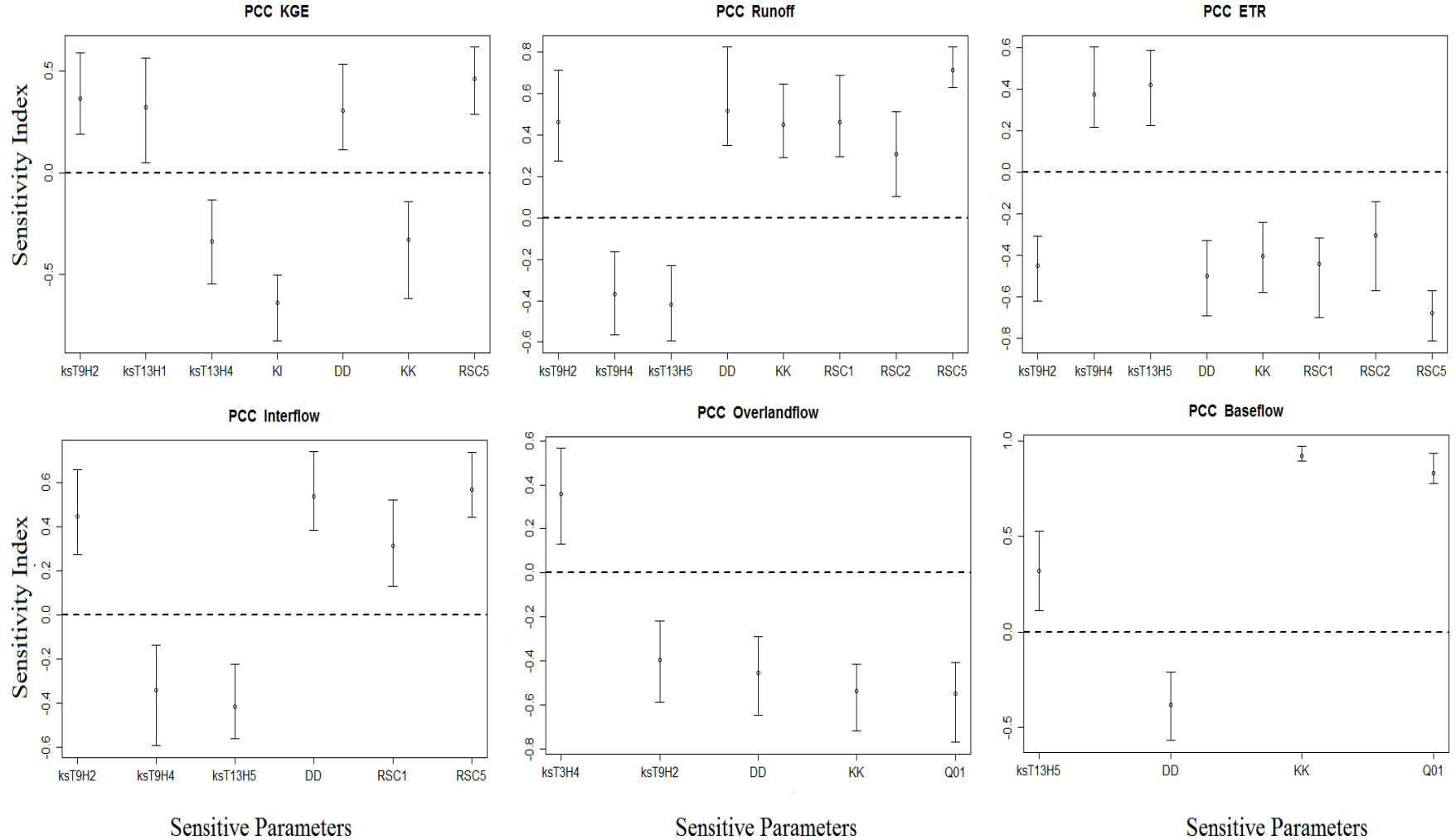
Figure 5-15: Sensitivity Index (corresponding to the partial correlation coefficient (PCC), see sub-section 5.3.2) for the most sensitive WaSiM parameters with absolute PCC greater or equal to 0.3. The uncertainty bounds and the real computed indices are represented for each sensitive parameter. The parameters are: the hydraulic conductivity of Albic Plinthosol (KsT9H2) and Mollic Gleysol (KsT13H1, KsT13H4), the interflow parameter KI, the drainage density DD, the leaf surface resistance of agriculture land RSC5, the baseflow parameters KK and Q01.
