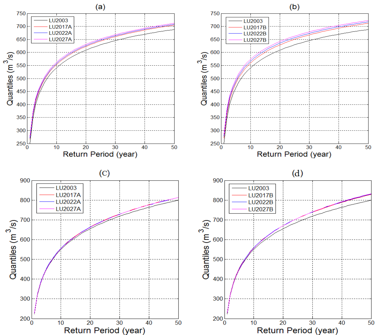
Figure 6-9: Quantile plots of the simulated discharges by WaSiM (a, b) and SWAT (c, d) for the different scenarios and the baseline.
