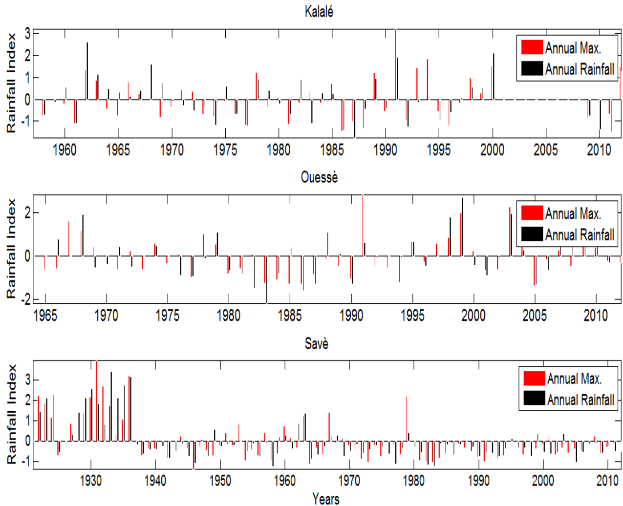
Figure 4-8: Standardized precipitation index (SPI) and standardized extreme precipitation index (SEPI) for three stations (Kalalé, Ouèssè, and Savè).
