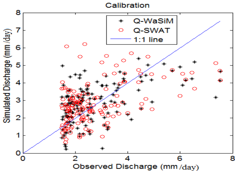
Figure 5-13: Scatter plot of the observed and simulated discharges by WaSiM and SWAT during the recalibration period.
