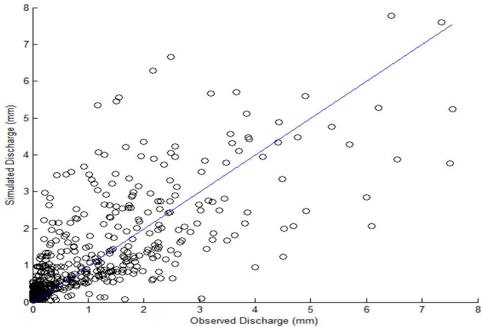
Figure 5-7: Scatter plot of the simulated discharge versus the observed discharge. The blue line represents the diagonal 1:1 with equation y=x .
