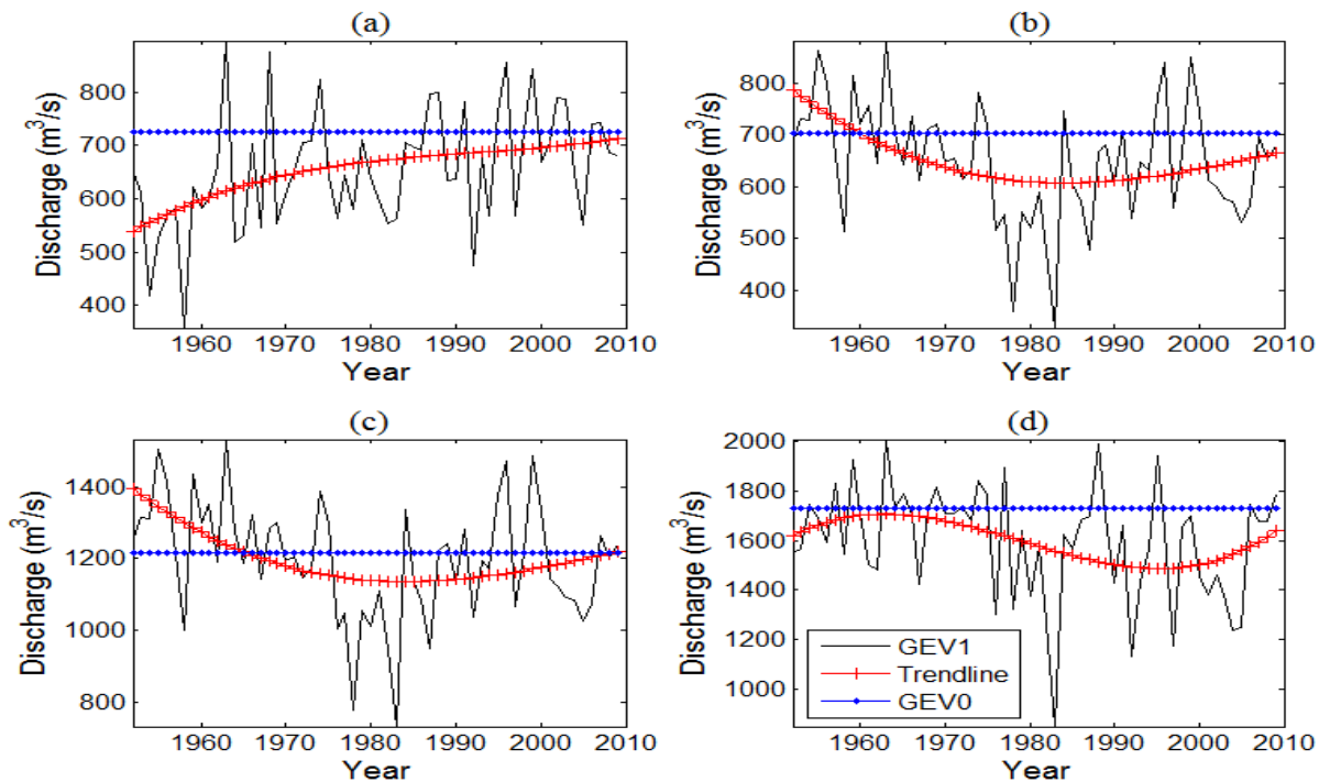
Figure 3-6: The 25-year effective flood values of the annual maximal discharge for the study period (1952–2009) at (a) Atchérigbé, (b) Bétérou, (c) Bonou, and (d) Savè based on the GEV1 (non-stationary) and GEV0 (stationary) models.
