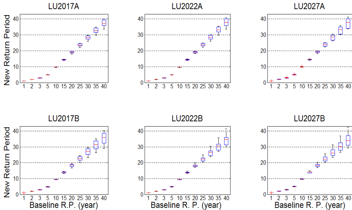
Figure 6-12: Baseline return period and the corresponding return period under the different land use scenarios and time windows for SWAT.
